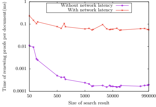
Figure 8. Performance of renewing proofs
