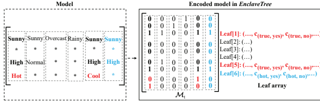
Figure 5: The model after one round training. The parts set in red are those modified after one round of training.
