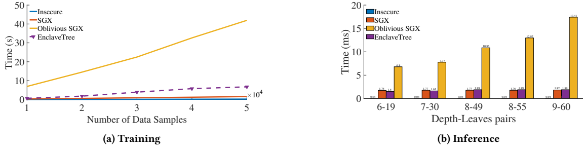
Figure 10: The Comparison of HT Training and Inference with 15 features
